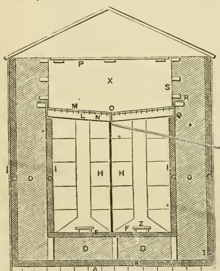
Fig. 27.—NYCE'S FRUIT PRESERVING HOUSE. (CROSS SECTION.)
